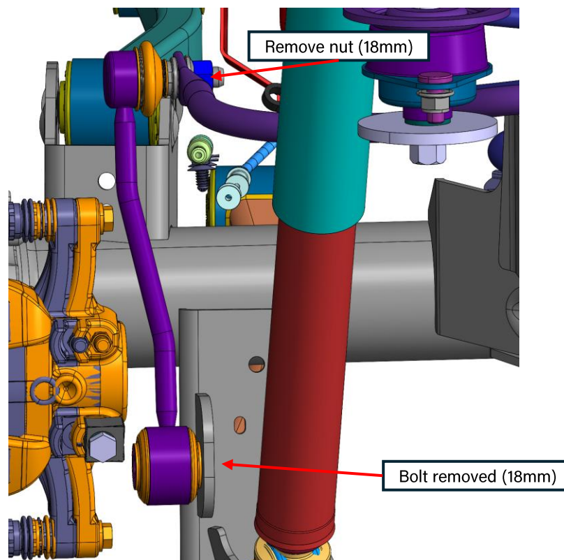
Figure 1: Driver-side Jeep JL rear sway bar to be removed (CAD photo)
