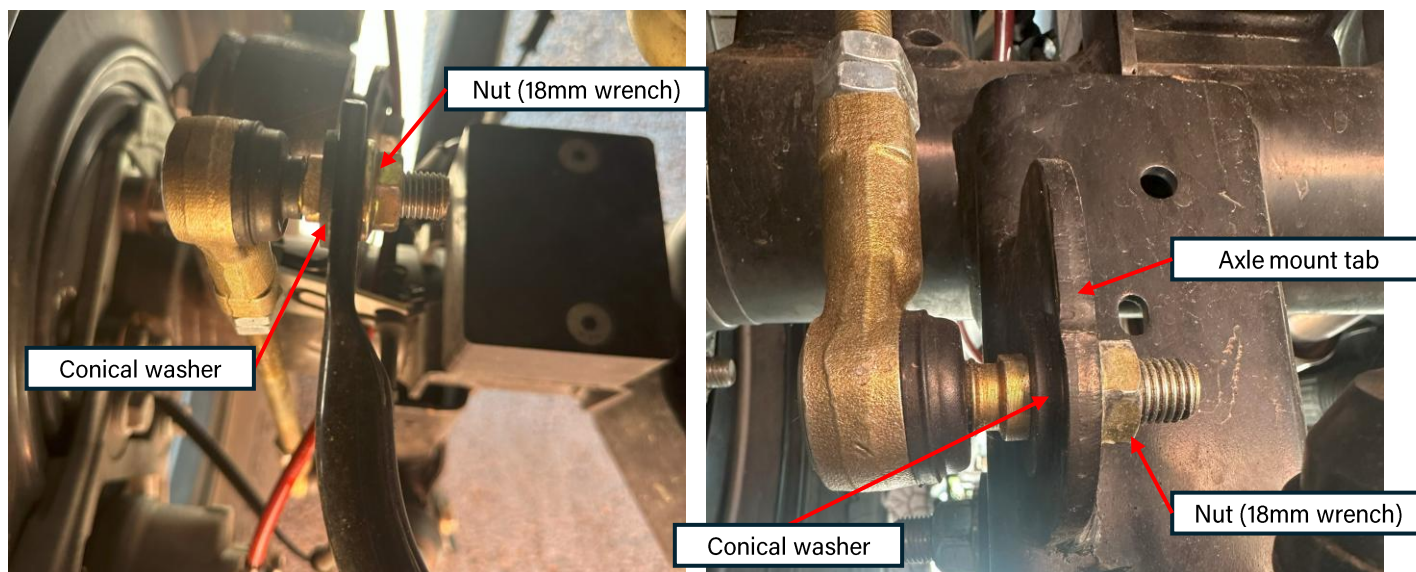
Figure 4: Sway bar end links installed on driver-side
