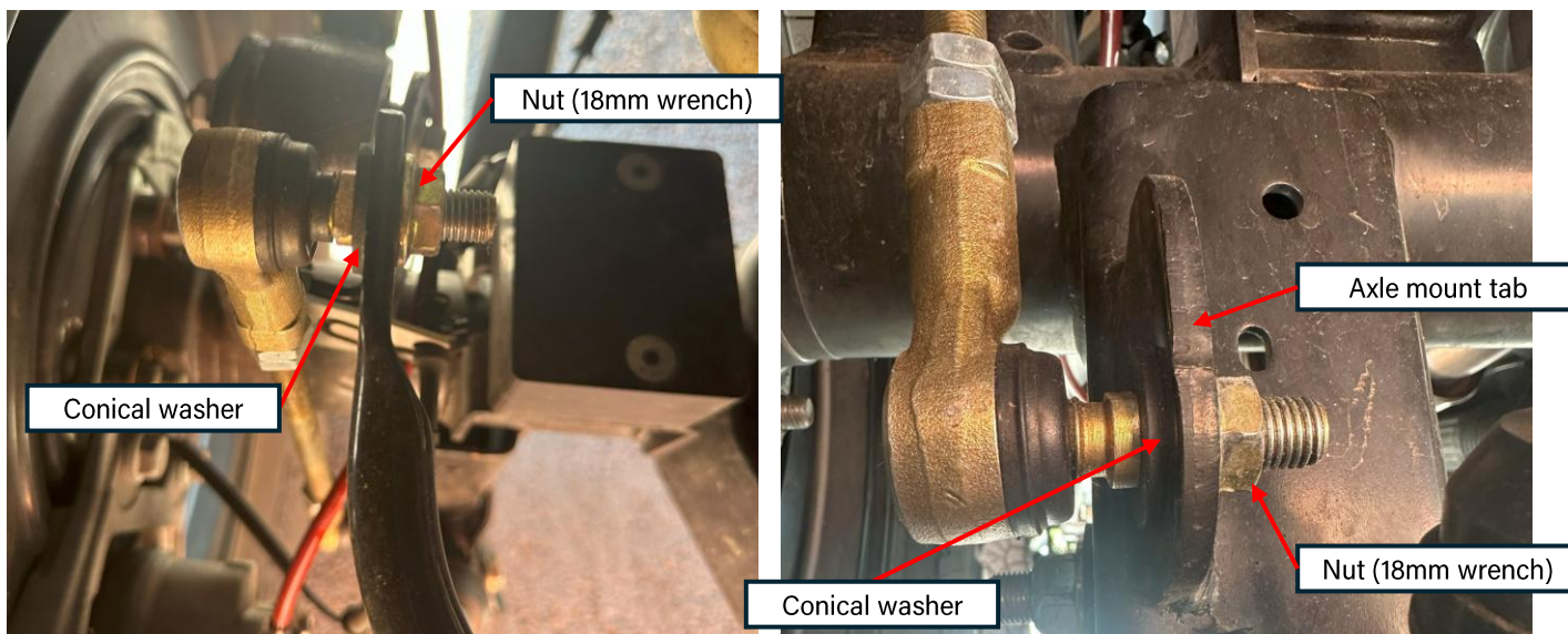
Figure 4: Sway bar end links installed on driver-side (rear of JL)
