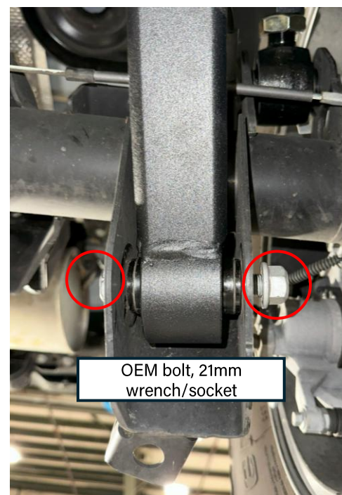
1709102 (OVERLAND+ Series) Rear lower control arm installed (frame-end and axle-end)
