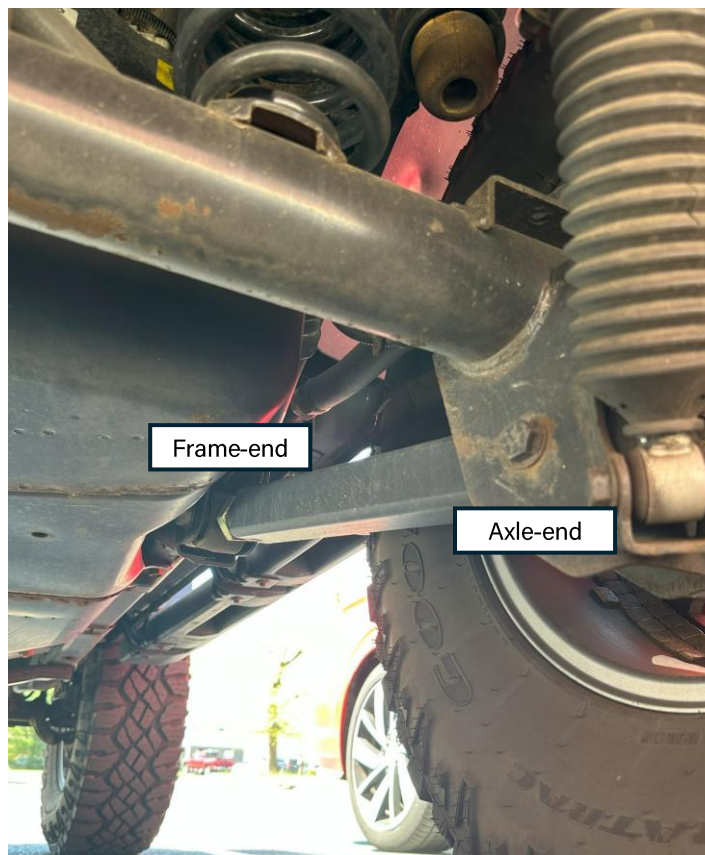
1709102 (OVERLAND+ Series) Rear lower control arm installed, passenger-side (Jeep JK)
