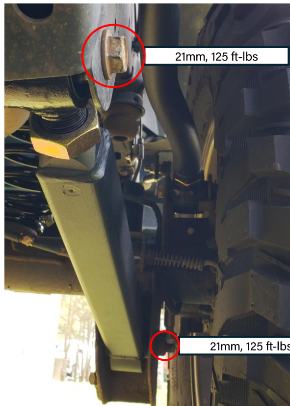
1709102 (OVERLAND+ Series) Rear lower control arm installed on Jeep JK
